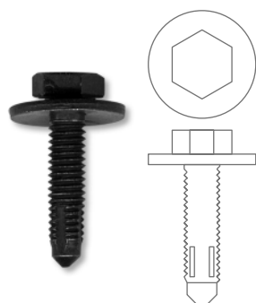
Tornillo Ø6 x 25mm, aro Ø18mm Aletas y parachoques P106, P1007, P306, P308, P406, P407, P607, Partner Cód. 0150.617.23
